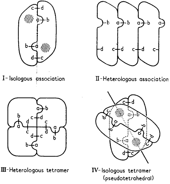
FIG. 8. Isologous and heterologous associations between protomers.
