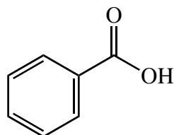
benzoic acid (mp 122°)
