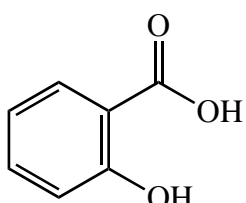
salicylic acid (mp 159°)
