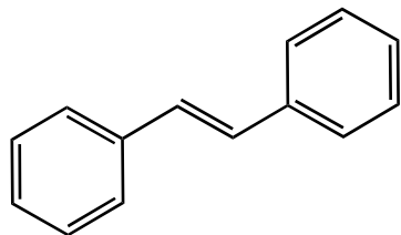
trans -stilbene (mp 125°)
