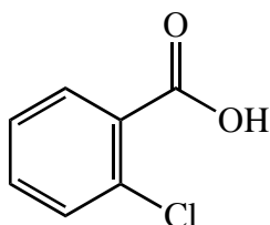
2-chlorobenzoic acid (mp 142°)
