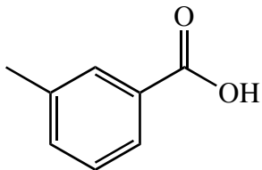
3-toluic acid (mp 112°)
