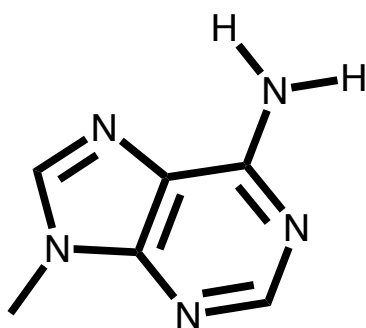
Adenine
