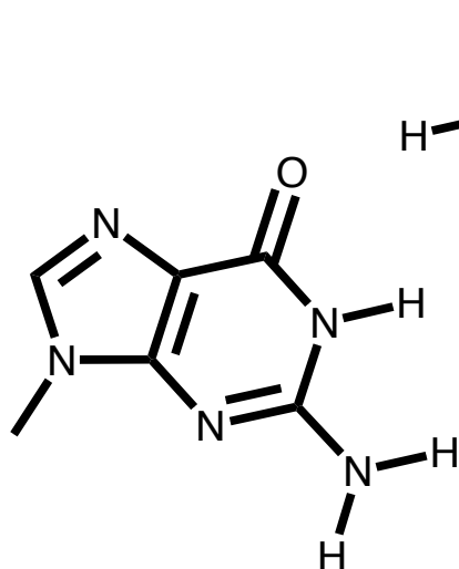
Guanine
