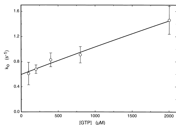
Figure 5. The dependence of the fit parameter k_{off} on the concentration of substrate GTP. Data presented are from Table 1.
