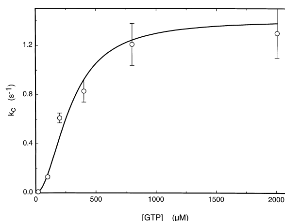
Figure 4. The dependence of the product formation step on the concentration of substrate GTP. Data presented are from Table 1.
