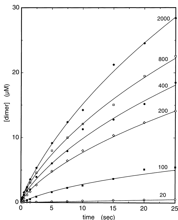
Figure 3. Production of dinucleotide pppGpG at various concentrations of substrate GTP (given in micromolar concentration above each data set). Conditions are given in Materials and Methods. Concentrations of enzyme and DNA are 5.0 and 3.0 \mu\text{M} , respectively.
