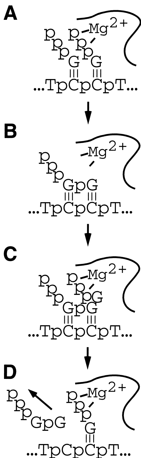
Figure 6. A model for substrate activation of product dissociation.
